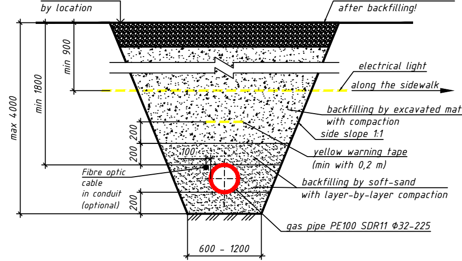
Gas pipe crossing electrical light that goes along the sidewalk
