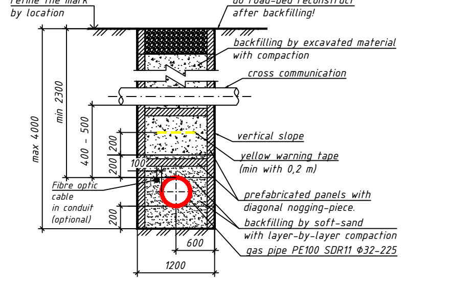
Trench with vertical slopes and prefabricated panels
