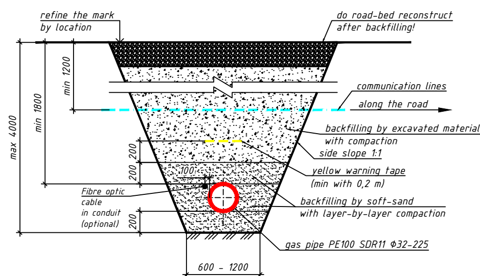
Gas pipe crossing communication lines that goes along the road
