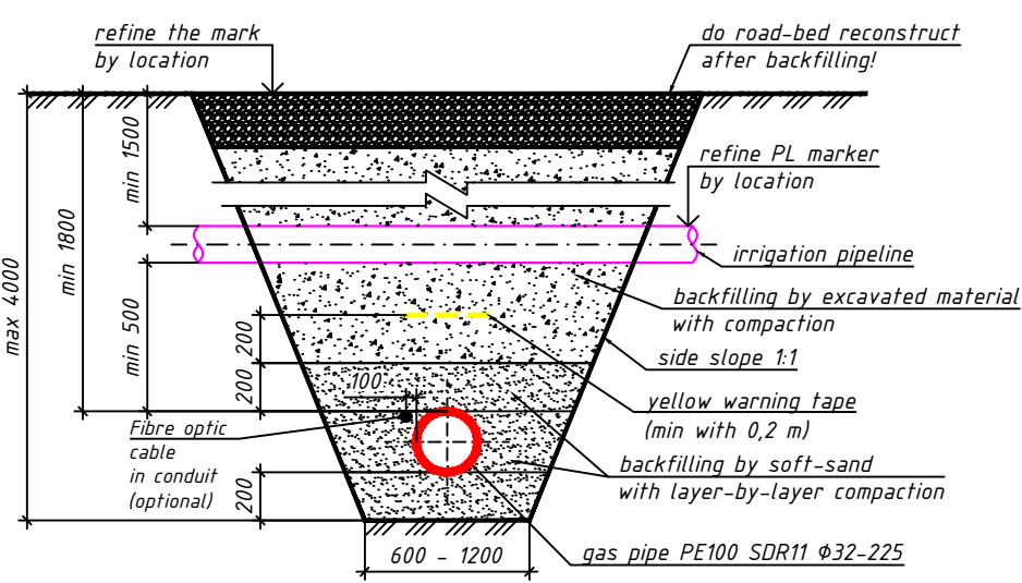
Gas pipe crossing irrigation pipe under it
