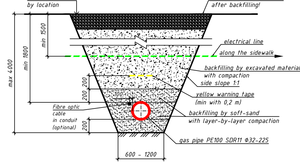
Gas pipe crossing electrical line that goes along the sidewalk
