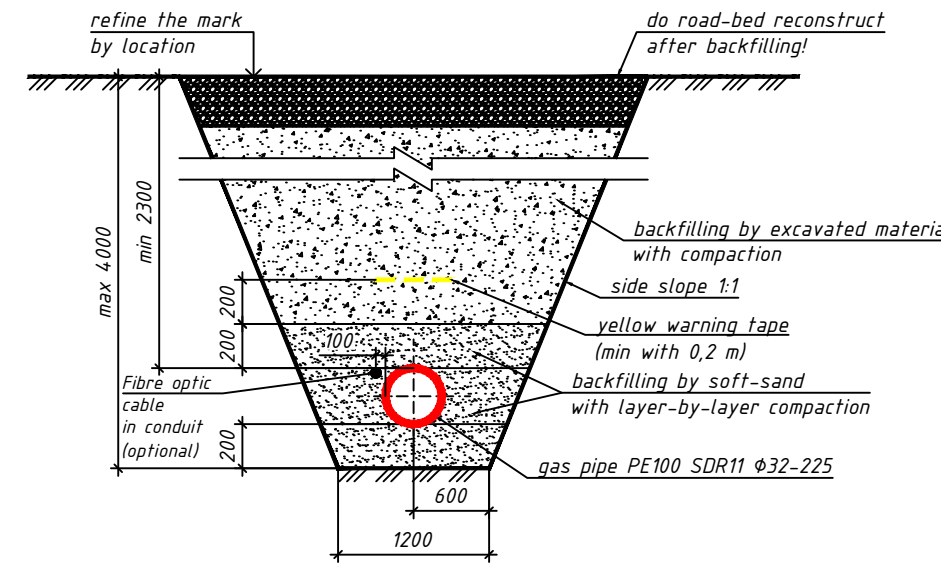
Without crossing communications (trench depth max 4000 mm)
