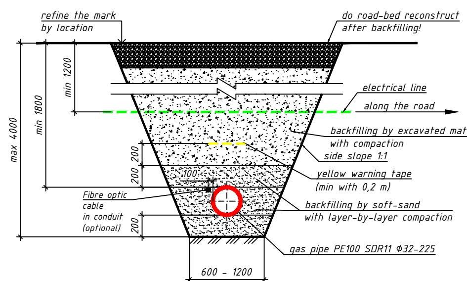
Gas pipe crossing electrical line that goes along the road
