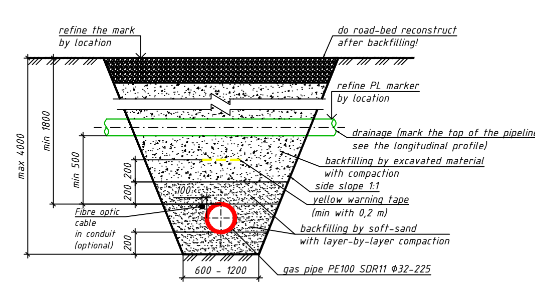
Gas pipe crossing drainage pipe under it
