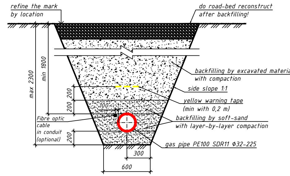
Without crossing communications (trench depth max 2300 mm)
