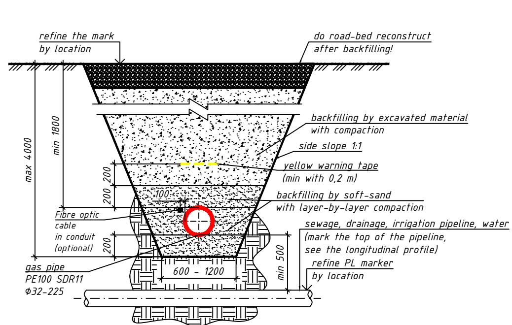
Gas pipe crossing communication lines that goes along the road
