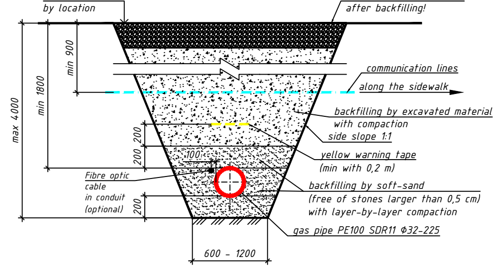
Gas pipe crossing communication lines that goes along the sidewalk
