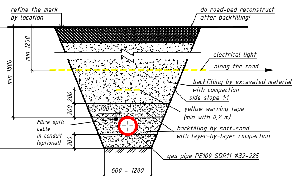
Gas pipe crossing electrical light that goes along the road
