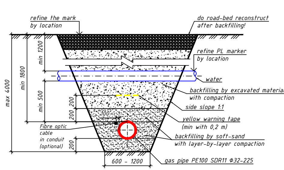
Gas pipe crossing water pipe under it
