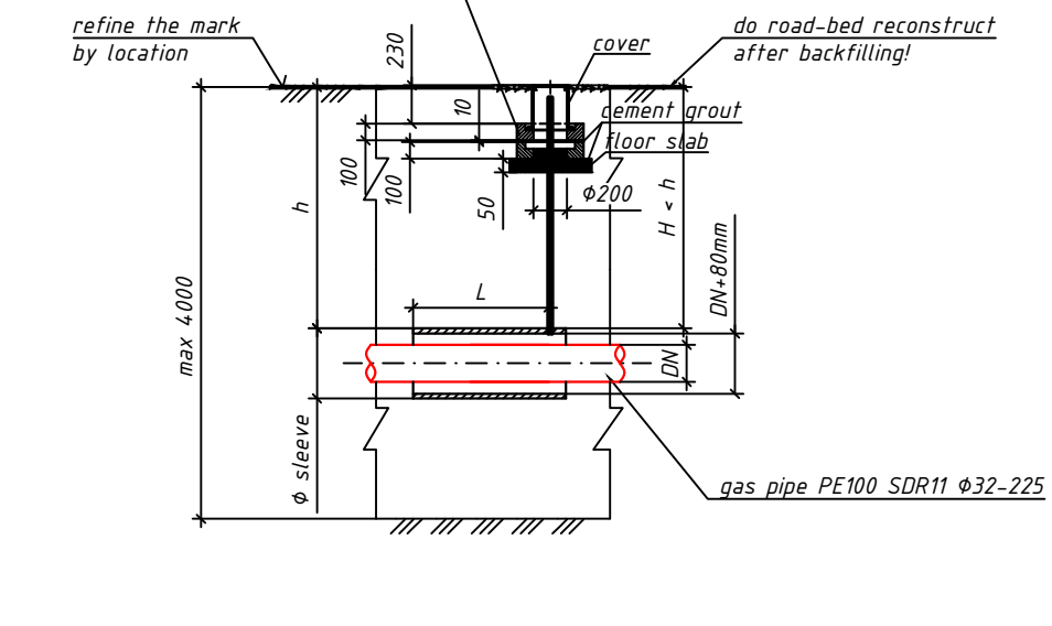
Covering control tube
