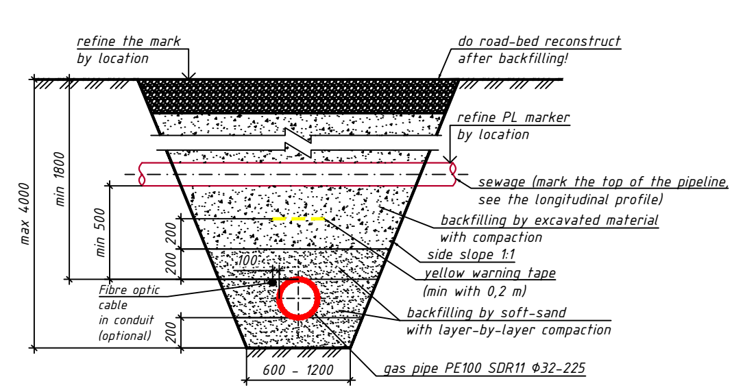
Gas pipe crossing sewage pipe under it
